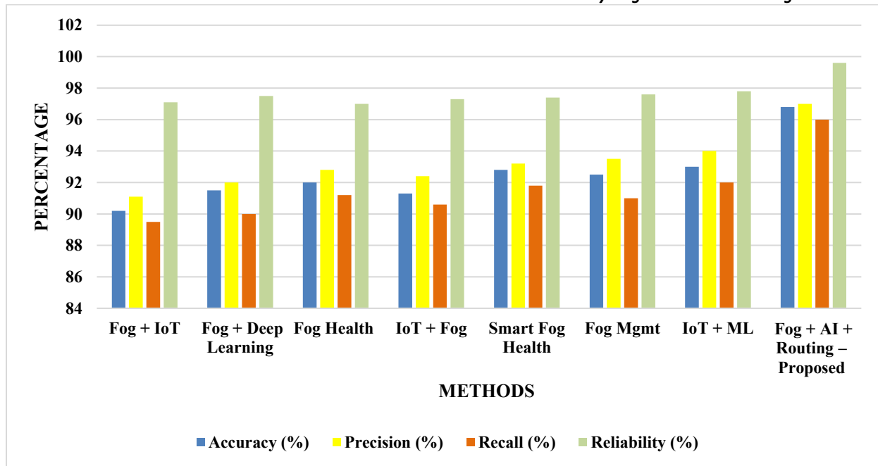
Figure 2: Performance Comparison of IoT-Driven Healthcare Systems Using Fog Computing, AI Models, and Data Routing Algorithms.
